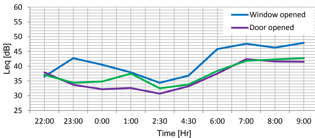
Figure 8: The back ground level measured during the night. The blue line indicated the measurements took place when a window was opened, the purple line indicates the situation when a door was opened and the green indicates a situation where both door and windows were closed.
